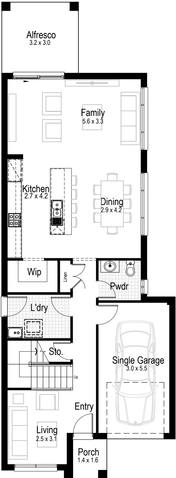
Ground Floor
