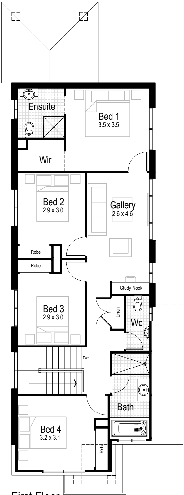
First Floor
